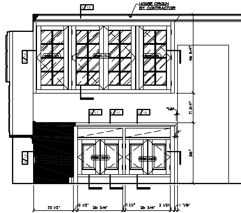
B EAST ELEVATION OF KITCHEN SCALE: 3/4" = 1'-0"
