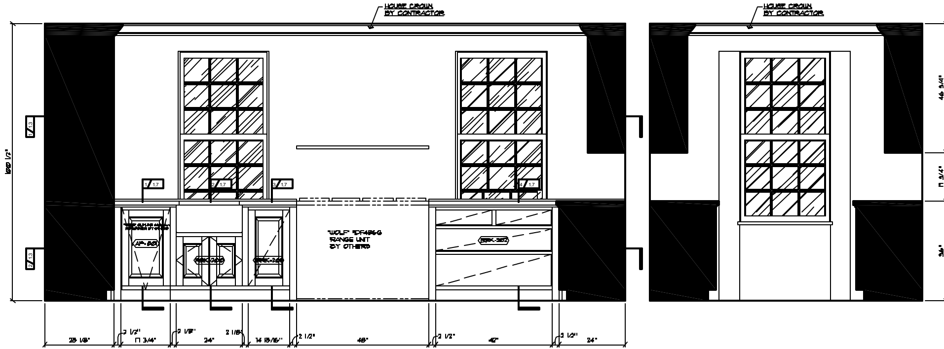
A NORTH ELEVATION OF KITCHEN & PANTRY SCALE: 3/4" = 1'-0"
